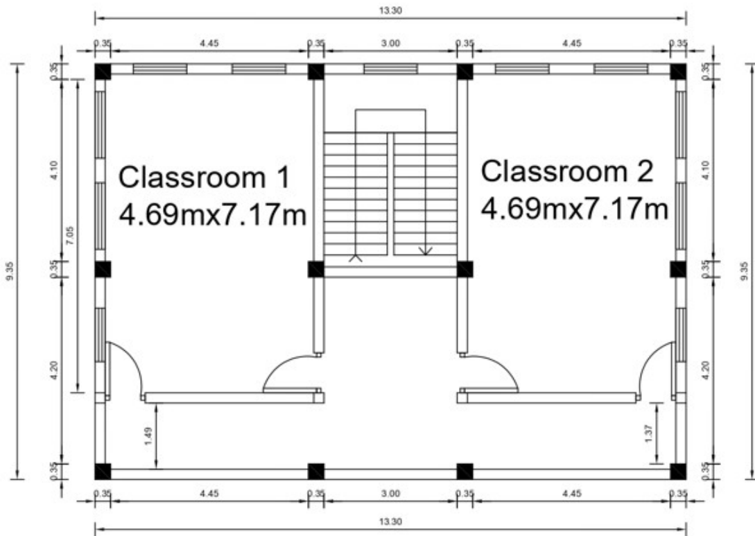
Ground Floor Plan 2 room building
